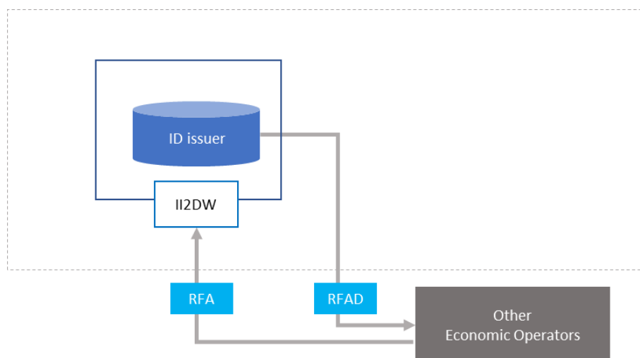
Figure 12 Issuing of a Facility Identifier code
