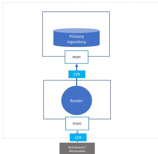
Figure 26 Data Flow Diagram – Receipt of payment – Report from Distributors and Wholesaler
