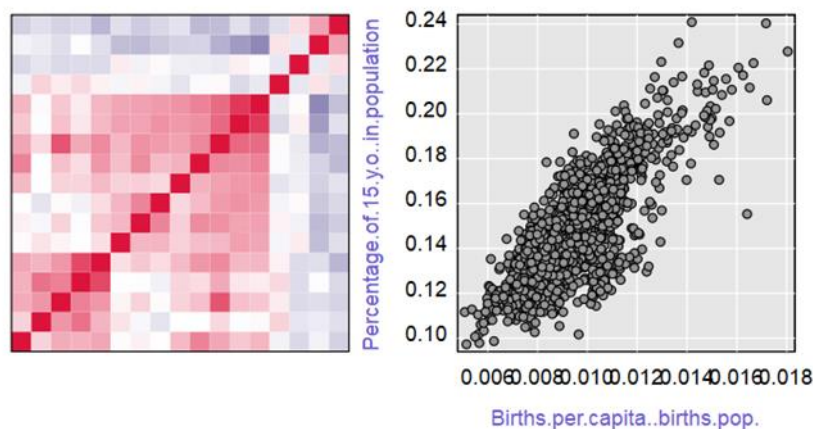
Figure 4 Correlation analysis with the statistical software R
